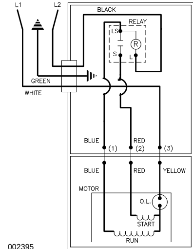
WIRING DIAGRAM FOR MODELS "N268-A", "N268-B", "N268-C", "N268-D" "E268-A", "E268-B", "E268-C", "E268-D" 4/82 (PN) to Current
