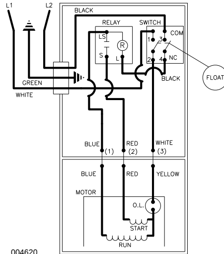
WIRING DIAGRAM FOR MODELS "M268-C", "M268-D", "D268-C", "D268-D" 9/86 (VS) to Current
